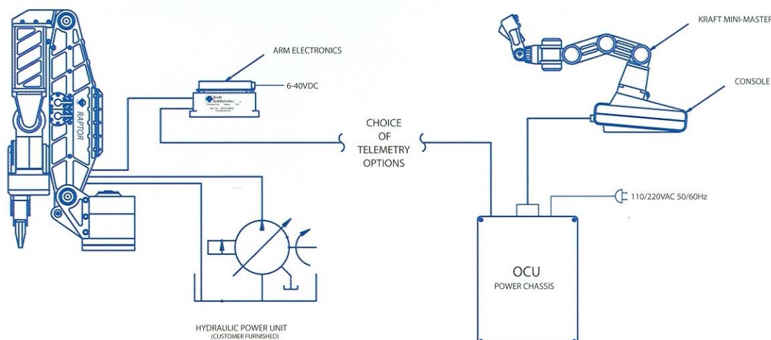
REMOTE MANIPULATOR ARM
