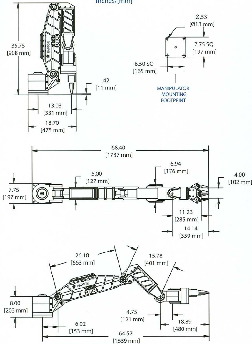
OUTLINE DRAWING Inches/[mm]
