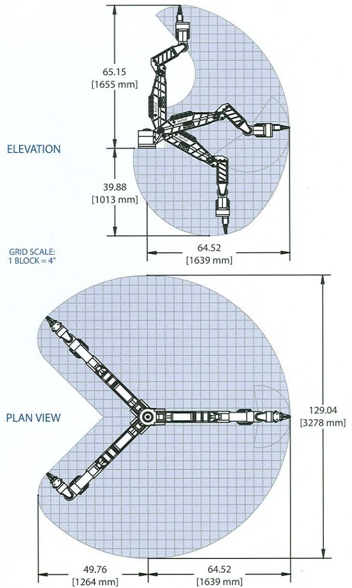
PERFORMANCE ENVELOPE
