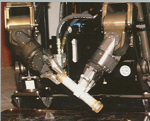
US Air Force "ARTS" vehicle, equipped with dual Raptor force feedback manipulator arms for the remote handling of unexploded ordnance.
